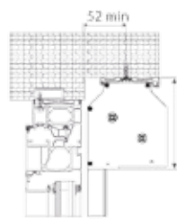
Mounting from down below with brackets
