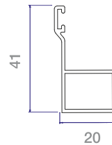
Casing Profile 20x41
