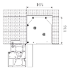
Self-supporting mounting let-in flush
