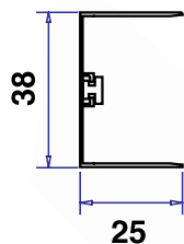
Magnet profile
