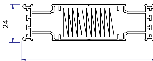
Mesh body
