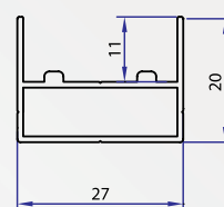
Bottom rail
