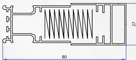
Mesh body
