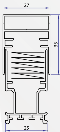
Mesh Body
