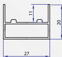
Bottom rail
