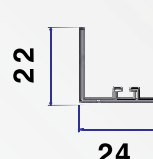
Magnet profile (single version only)
